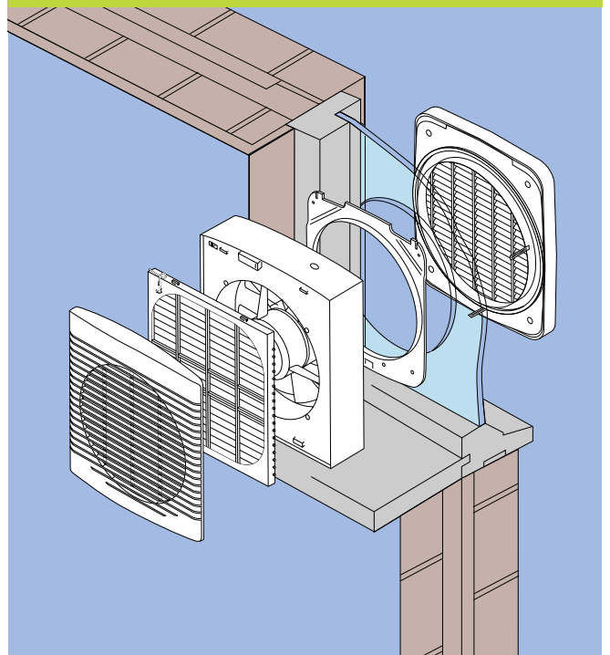
GX9/12 WINDOW MOUNTED UNIT
