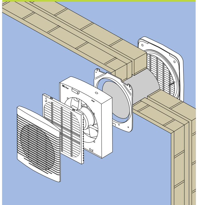
GX9/12 WALL MOUNTED UNIT
