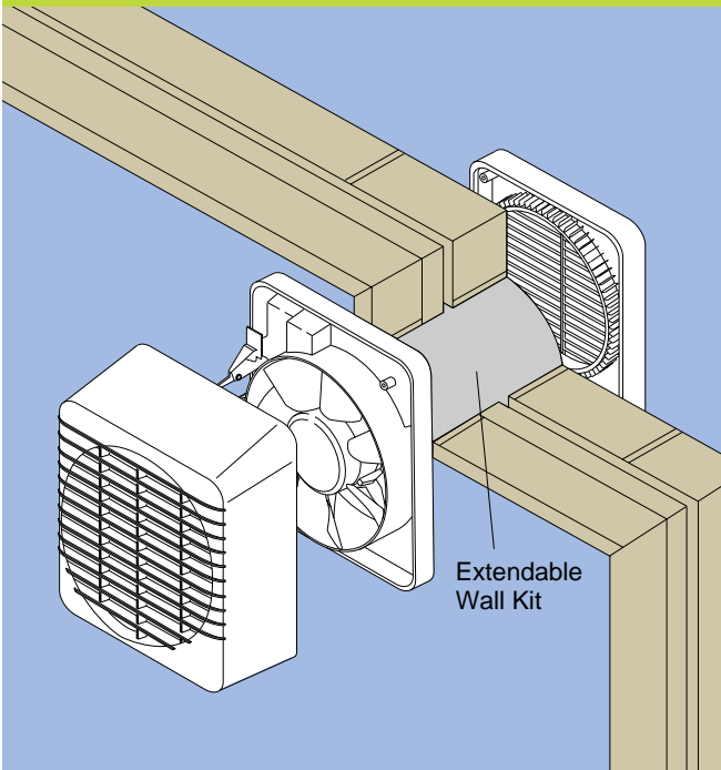
GX6 WALL MOUNTING
