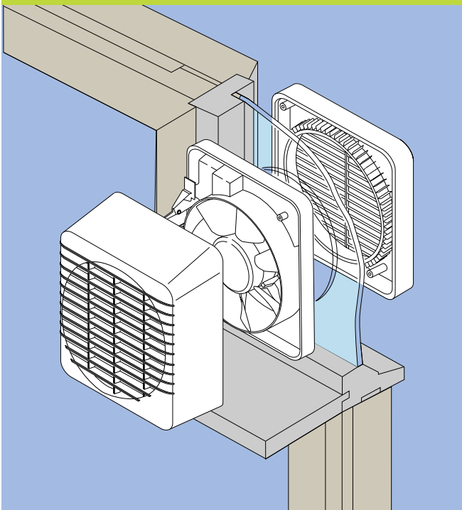
GX6 WINDOW MOUNTING
